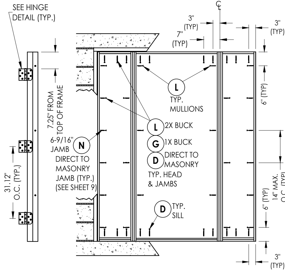
HINGE MULLION
