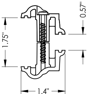
3A ODL LITE FRAME HP Polypropylene 1/2" I.G.
