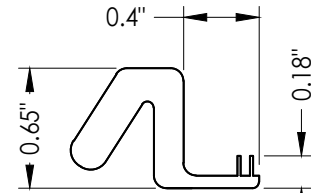
7 WEATHERSTRIP
