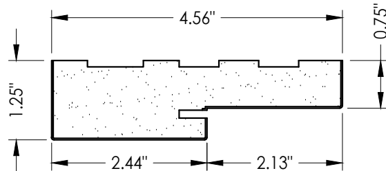
18 OUTSWING THRESHOLD By Endura
